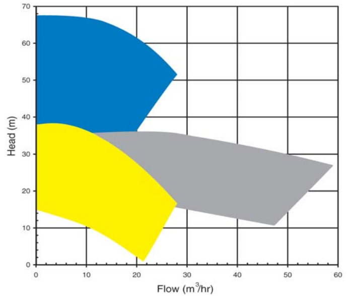
2900 rpm, 50 Hz
