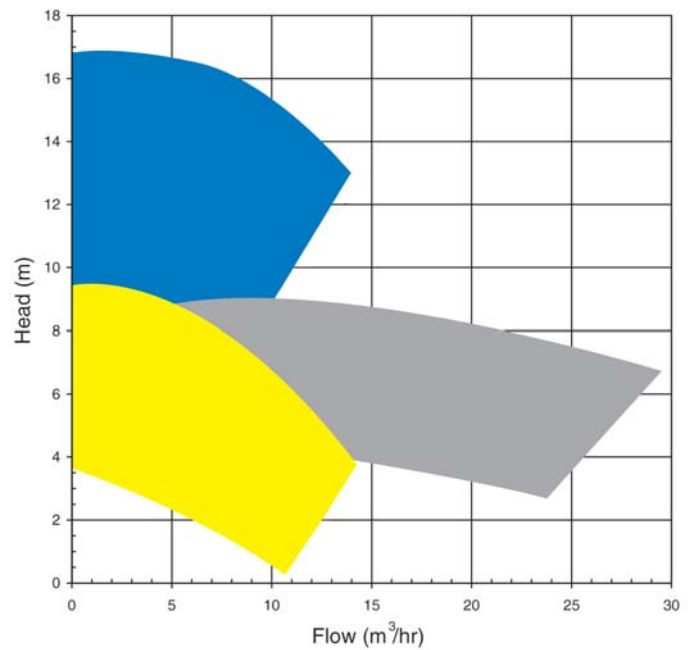
1450 rpm, 50 Hz
